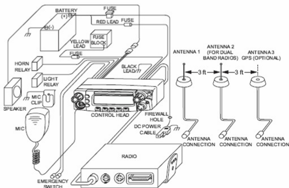
Figure 2-6. Radio Installation (O5 Mid Power Remote Mount)
